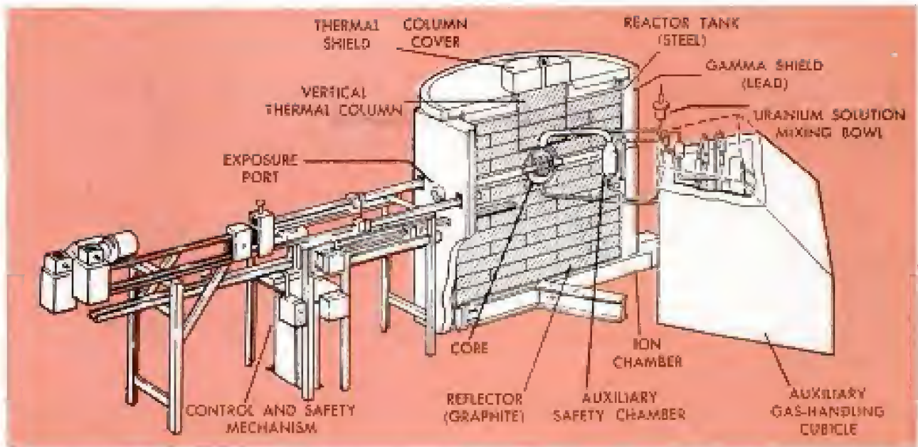
Core of the "tea kettle" is filled with uranium solution. Safety rods run through it to control the fission
